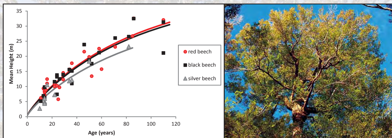
Figure 1: Mean height of beeches in plantations aged between 10 and 110 years.
