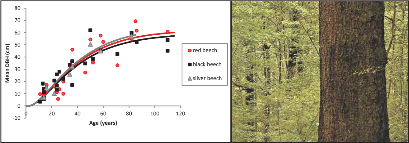
Figure 2: Mean diameter of beeches in plantations aged between 10 and 110 years.
